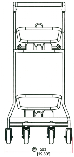
VIEW "A"
